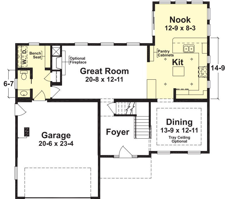
Greenfield 1st Floor 47'-0" x 47'-6", 2272 sq ft
