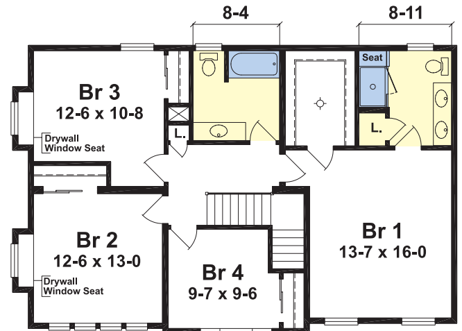
Greenfield 2nd Floor Optional 4th Bedroom
