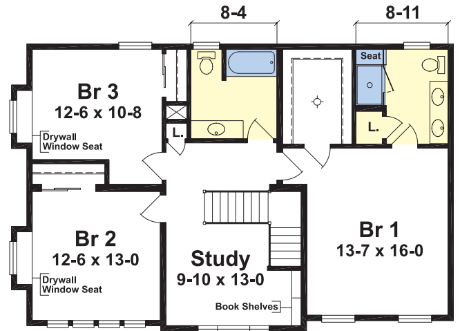
Greenfield 2nd Floor 27'-6" x 42'-6" 3 Bedroom Plan
